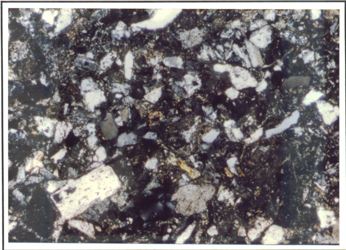
Figure 1: GC333-1, Tarra-1, Core 2. Strzelecki Group Volcanogenic sandstone. Compacted texture due to high proportion of ductile volcanic rocks fragments (VRF's). Diagenetic swelling chlorite/chlorite grain coatings well developed. Feldspars albitized. Laumontite (zeolite) well developed. A. Plane polarised light Width of field of view = 2.20 mm B. Crossed polarised light Width of field of view = 2.20 mm
