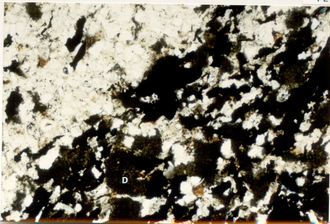
Figure 12: SWC 30, 2807.5m, 2mm, PPL Part of a bed of opaques and carbonate aggregates. The latter are dark, mottled, e.g. at D. The remainder of the rock is an impervious fine-grained sandstone.
