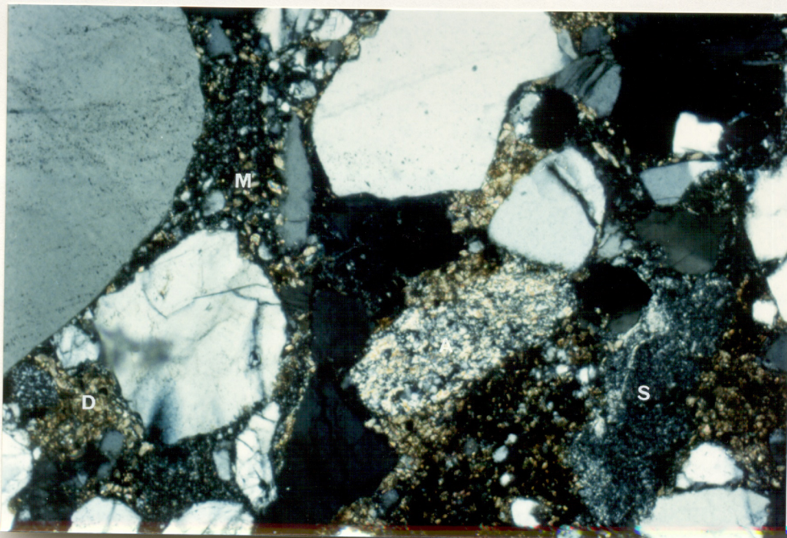
Figure 11: SWC 24, 2908m, 2mm, CL Siliceous (S) clast and schistose clast (A), dispersed matrix (M) and patches of authigenic carbonate (D) are present in this field-of-view.
