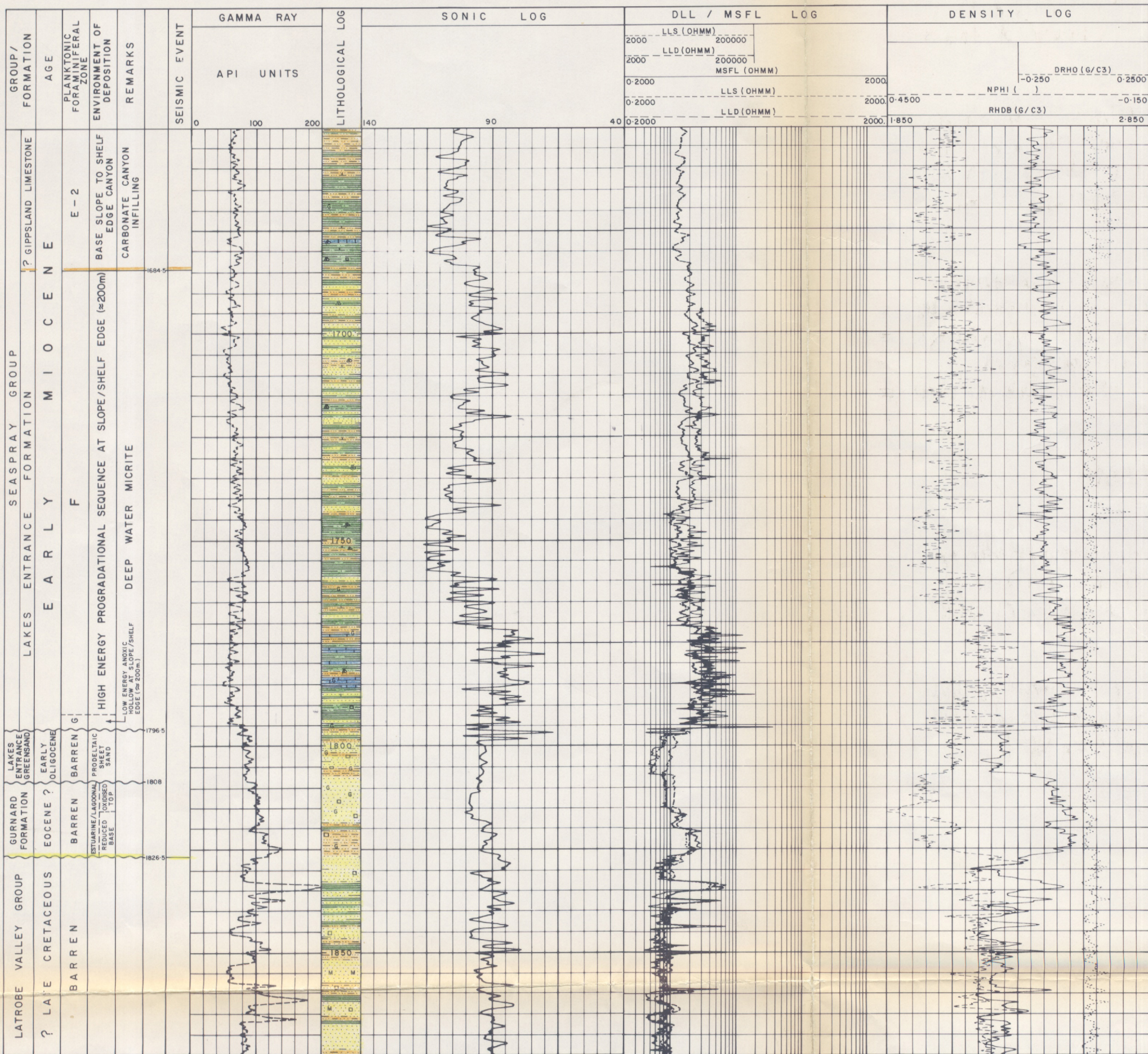
FIGURE 5 : PISCES No. 1 : DETAILS OF THE SECTION 1650 - 1875 m. (b.k.b.)
