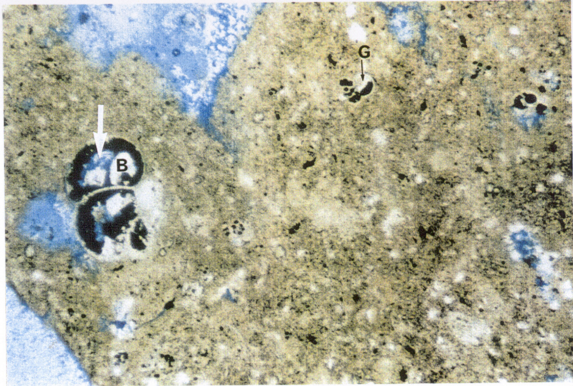
Figure 16. Thin section photomicrograph of fossiliferous micrite. Primary intragranular pores (arrow) are present. Foraminiferal tests are partially filled with pyrite, oxidised glauconite (G) and ?barite (B). Mudskipper #1, depth 1557.0m. Plane light. Field of view 0.88mm.
