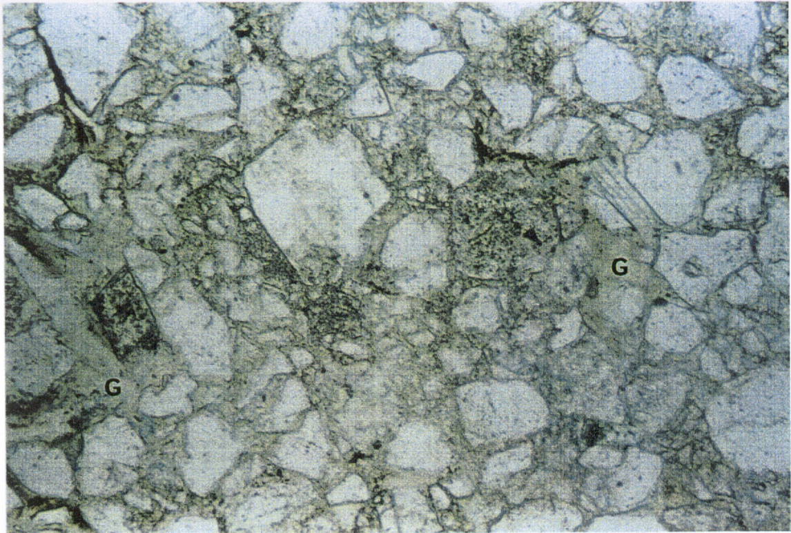
Figure 8a. Thin section photomicrograph of pale green and brown pore filling chlorite (G). Mudskipper #1, depth 1600.5m. Plane light. Field of view 0.88mm.
