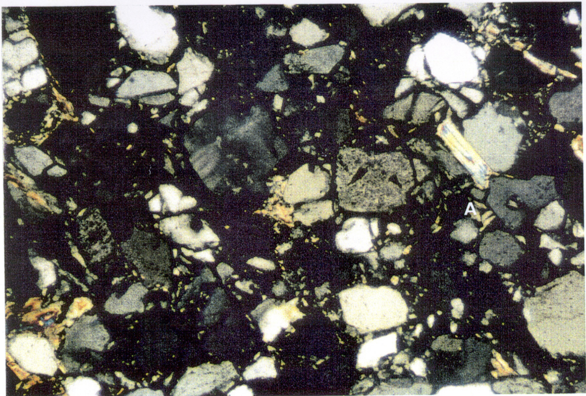
Figure 8b. Same field of view as Figure 8a in crossed nicols. Chlorite is commonly composed of radiating, anhedral booklets (A).
