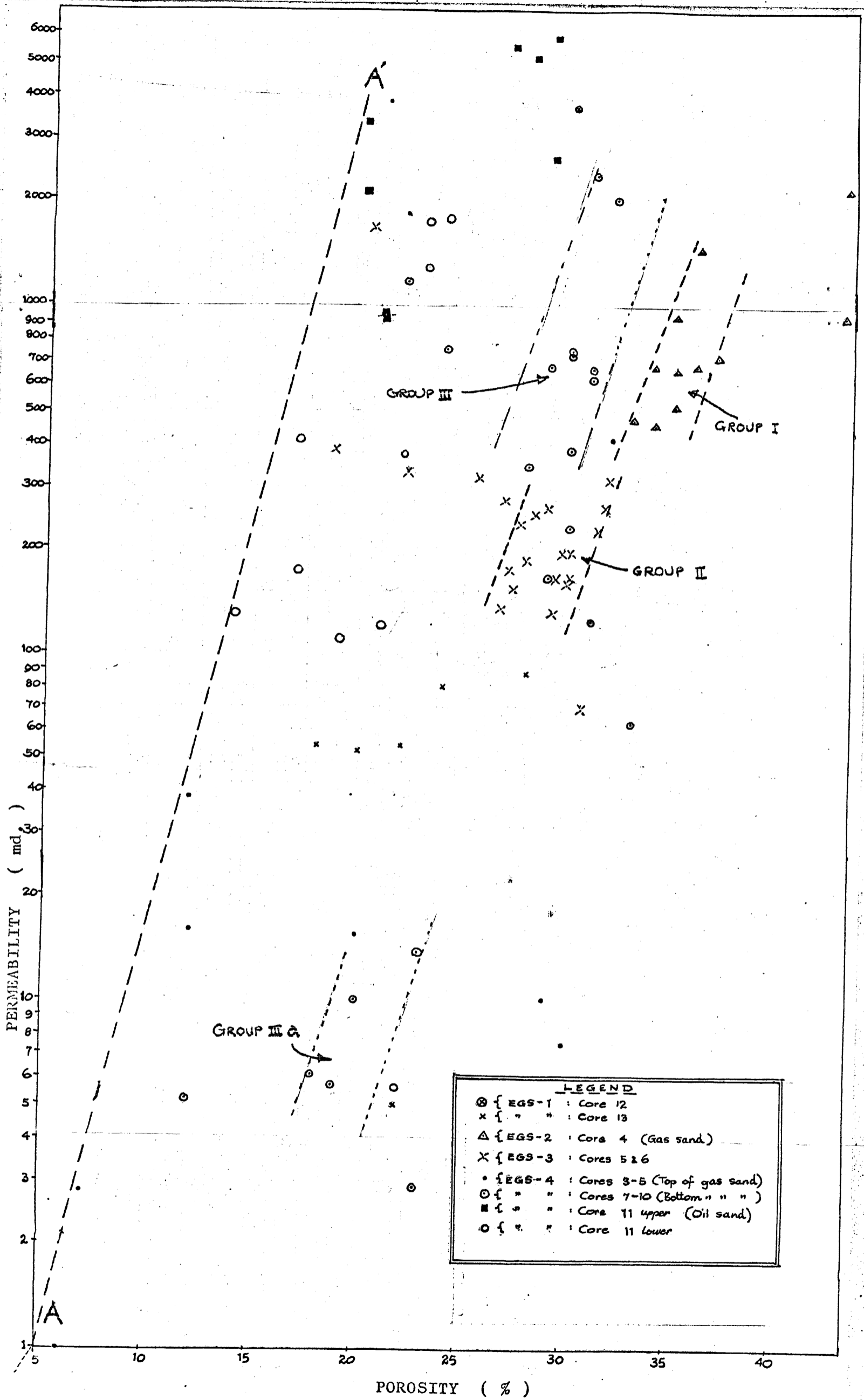
FIG. 3 RELATIONSHIP BETWEEN POROSITY AND PERMEABILITY
