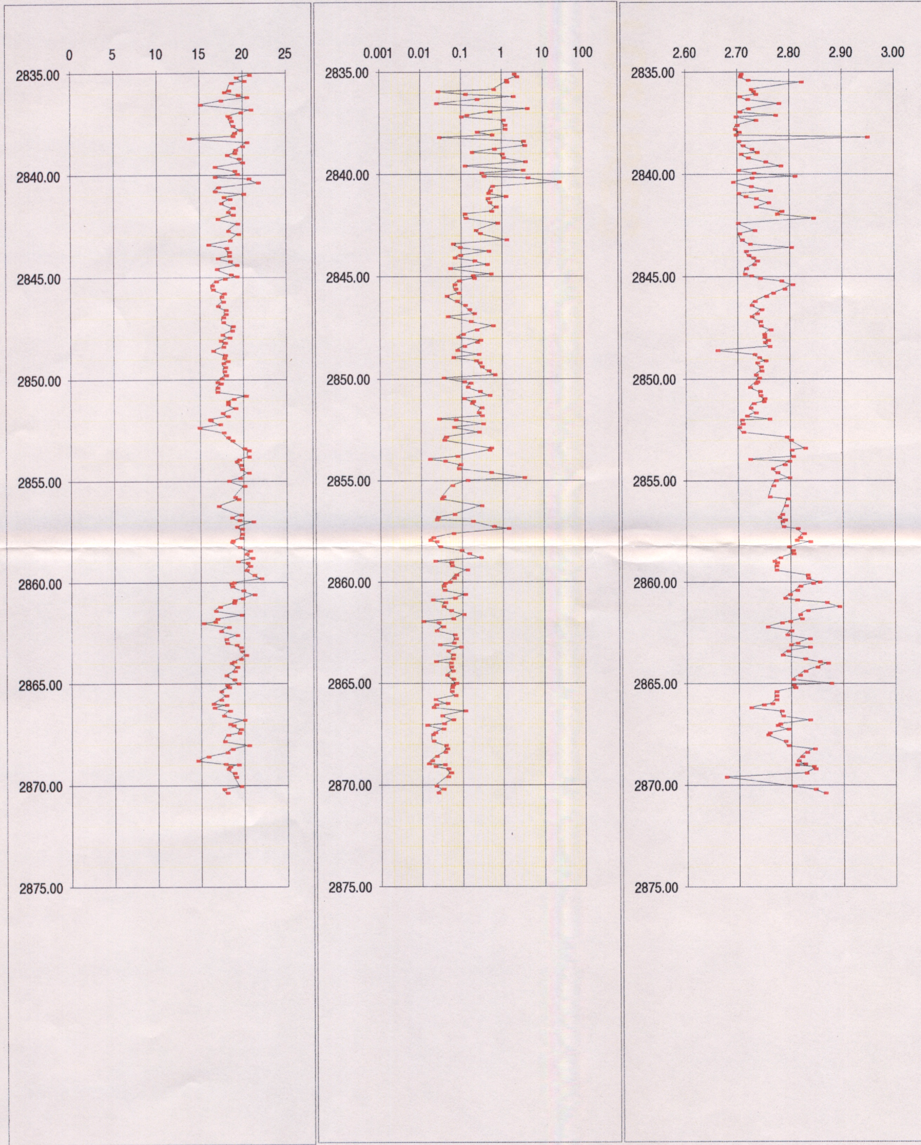
Porosity (%) vs Depth(m)
