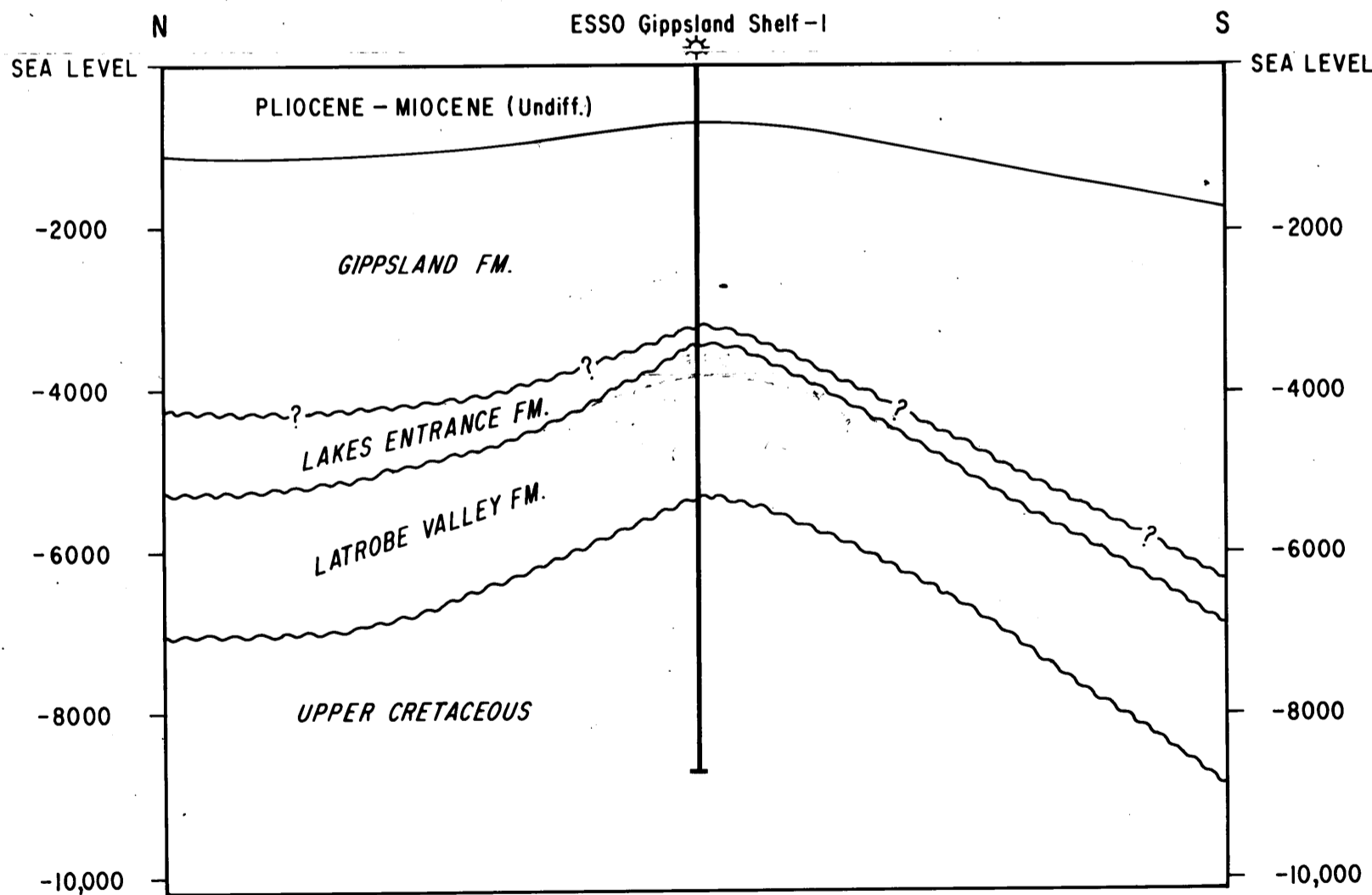
CROSS - SECTIONS BEFORE AND AFTER DRILLING ESSO GIPPSLAND SHELF - 1
