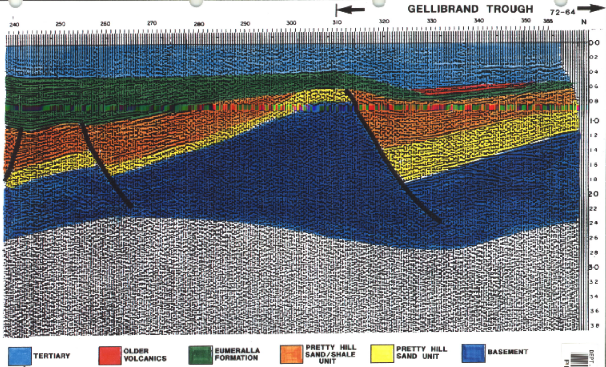
FIGURE 6 - SHELL SEISMIC LINE 72-64 SHOWING THE SOUTHERN PORTION OF THE GELLIBRAND TROUGH
