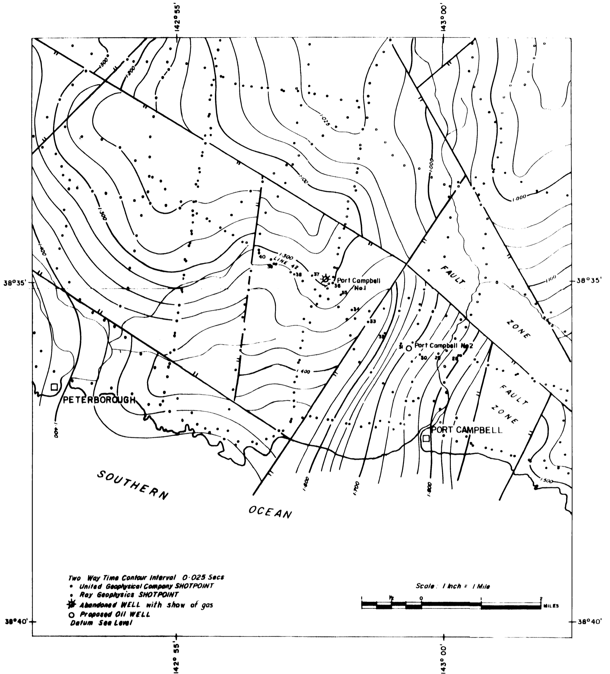
FROME-BROKEN HILL CO. PTY. LTD. PORT CAMPBELL No 2 SEISMIC CONTOUR MAP—TOP OF WAARRE FORMATION. PRIOR TO DRILLING.
