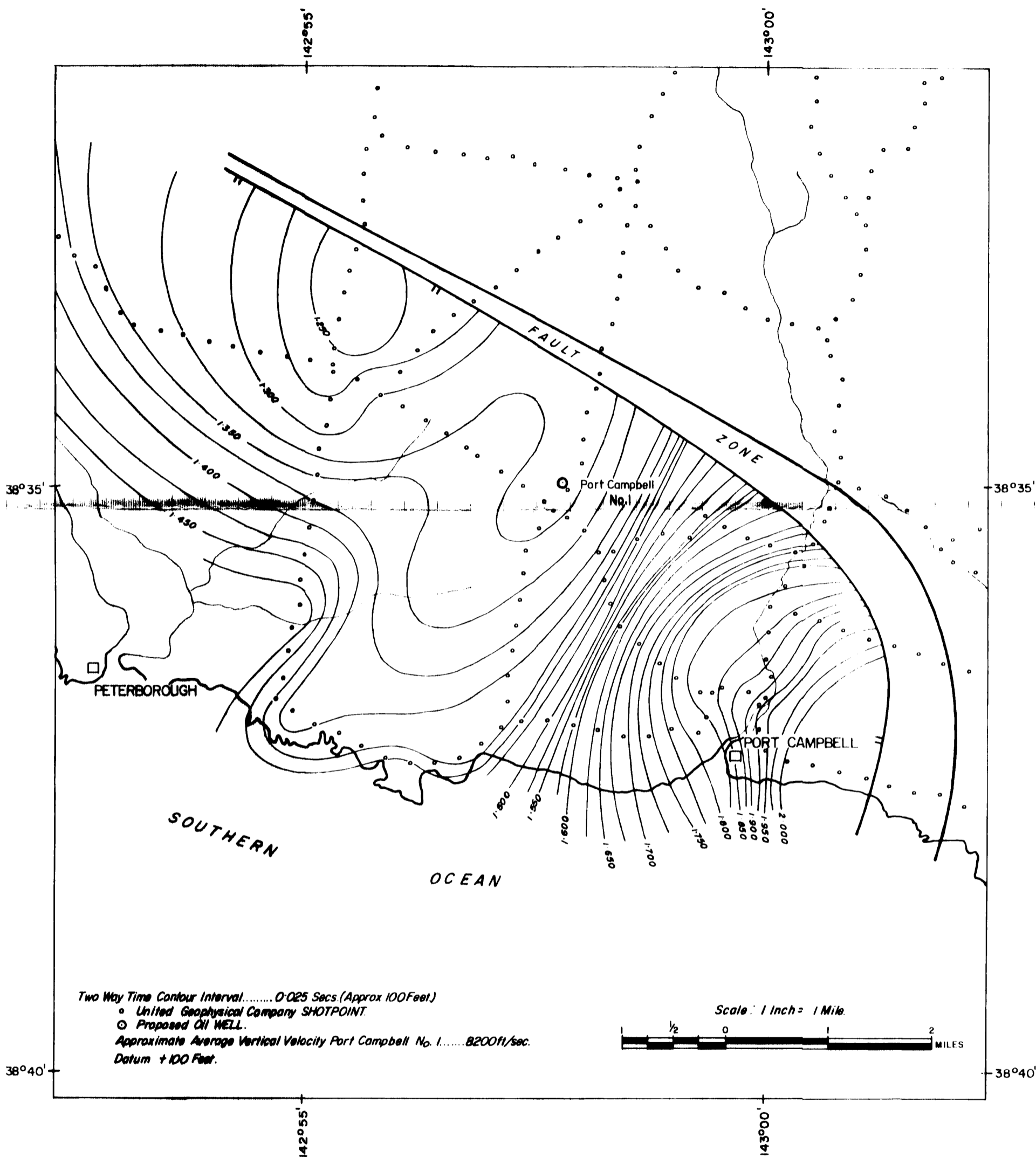
FROME-BROKEN HILL CO. PTY. LTD. PORT CAMPBELL No. 1. SEISMIC CONTOUR MAP — TOP OF JURASSIC PRIOR TO DRILLING.
