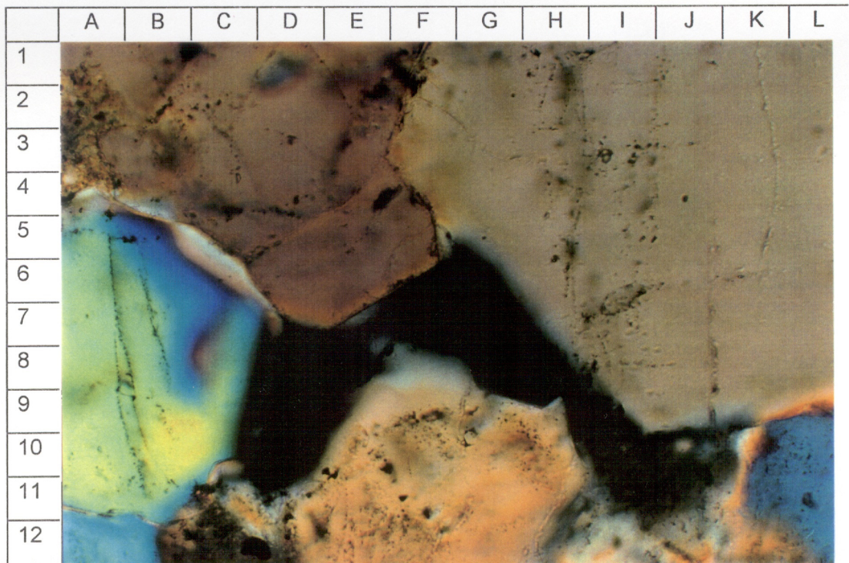
Figure 2B Rare example of quartz overgrowth development (e.g. E:7 & F:8). Veilfin-1, 3405-10 m ctgs sample, transmitted light with cross nicol (100 \mu\text{m} = 17.5 mm).
