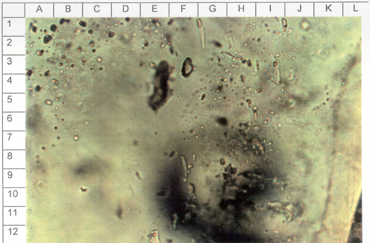
Figure 6B Same subject as 6A taken in transmitted light. Note the low refractive index of the dark gas bubble in the inclusion at F:3. Inclusions containing mostly gas could either represent condensate or mixing of oil and gas.
