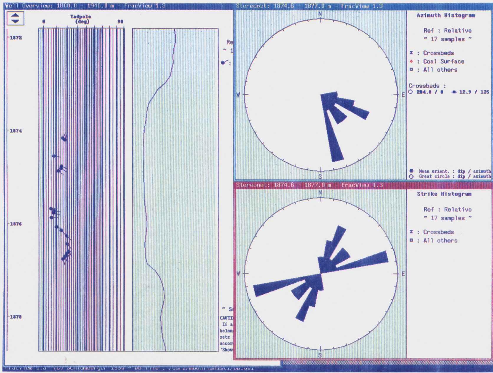
FIGURE 5 Crossbeds SDR Dip Azimuth 135° Interval 1874m to 1877m.
