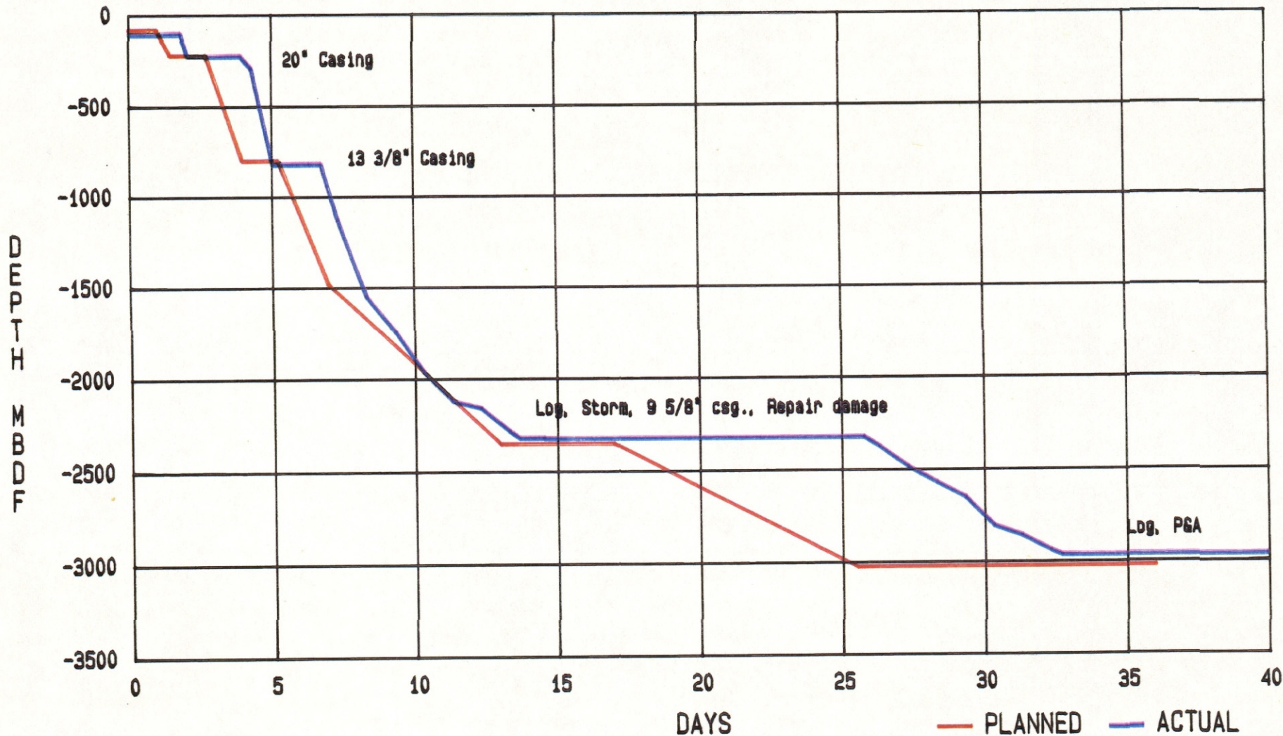
Figure 2 TIME VS DEPTH CHART - JUDITH-1
