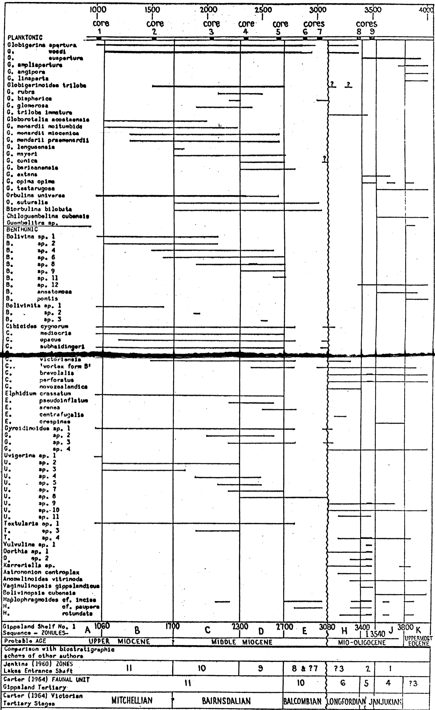
Figure 1 - TERTIARY FORAMINIFERAL DISTRIBUTION
