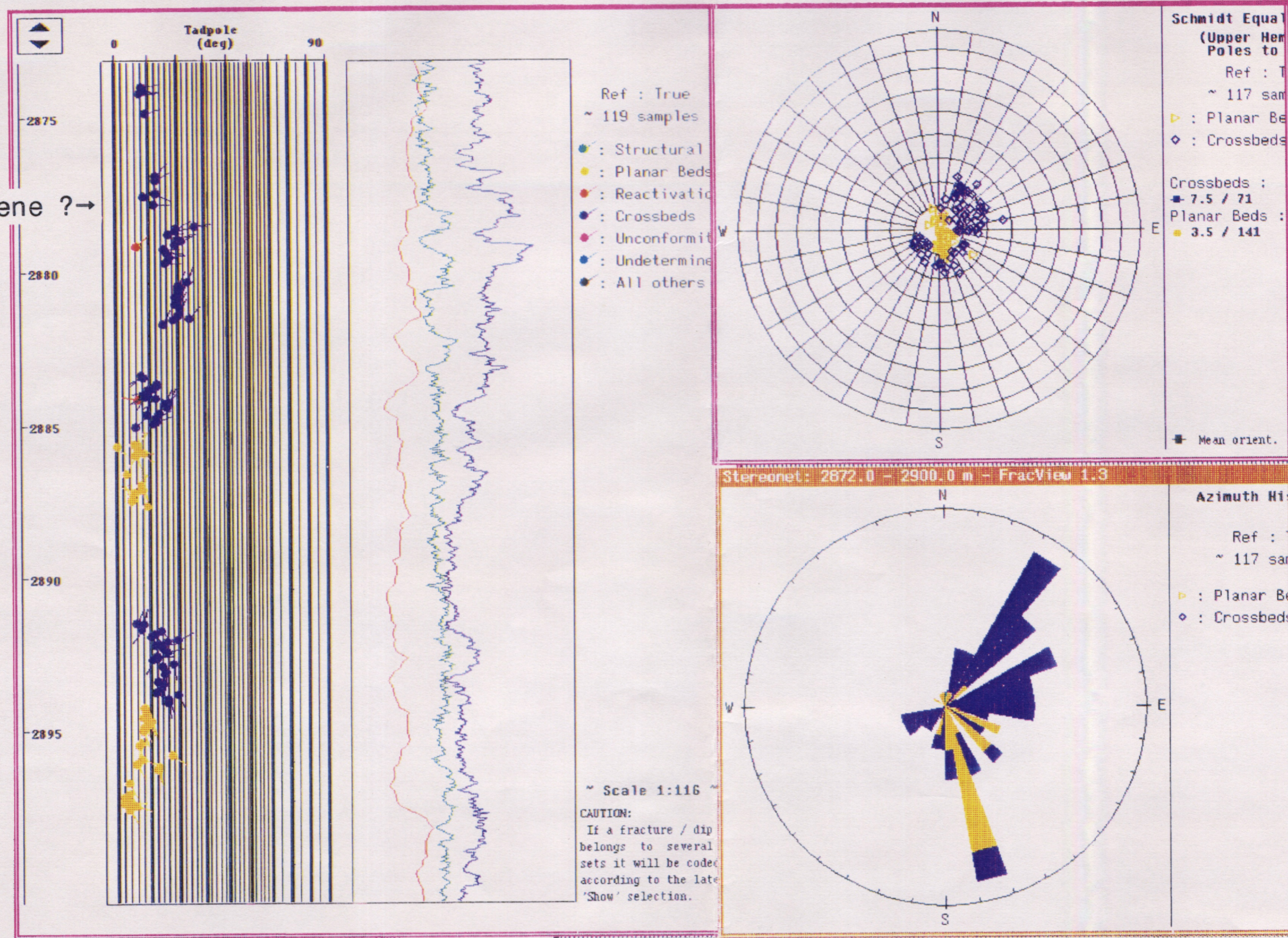
Figure 6 2873m to 2900m Paleocene age stratigraphy trough crossbedding and low angle planar bedding. Planar beds: Dip 3.5° Azi SE Crossbeds: Dip 6°-20° Azi NE
